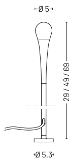
Mounting by plate
