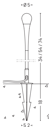
Mounting by spike
