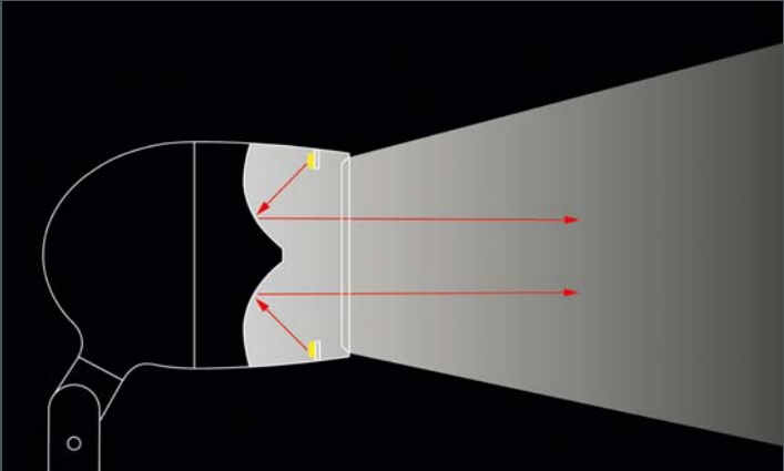
With the innovative Darkring optic light from a circular LED board is projected onto the target area via an indirect reflector. The light source is shielded from view and excellent glare control is achieved.
